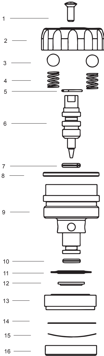
Figure 4 - Compression valve assy
