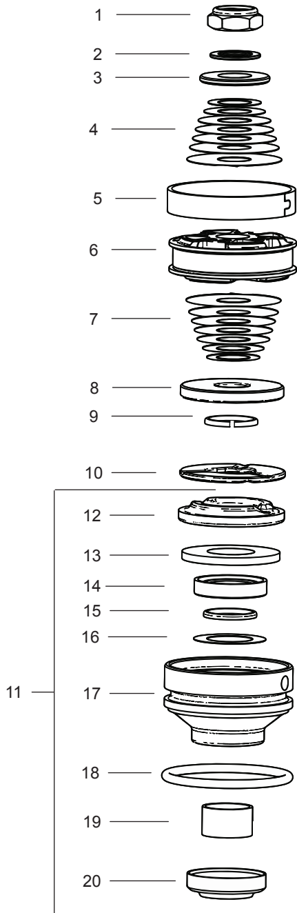
Figure 3- Damping assy+Seal head assy
