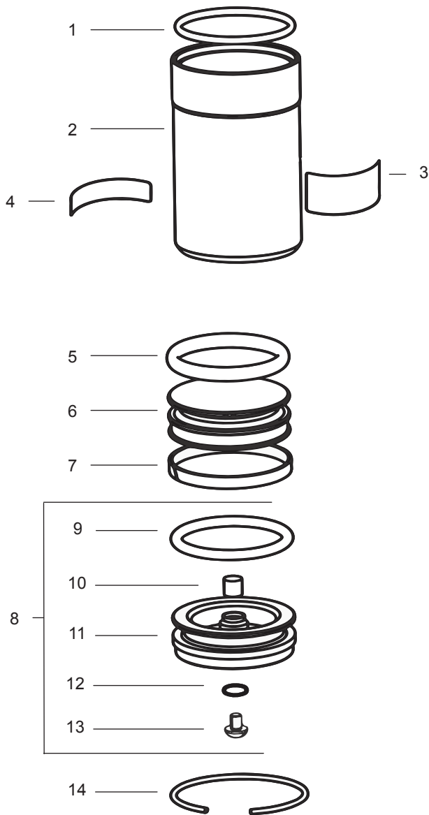
Figure 5 - Reservoir assy
