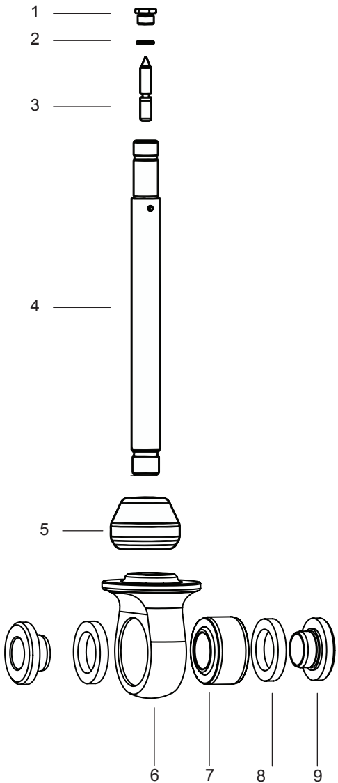
Figure 2 - Shaft assy
