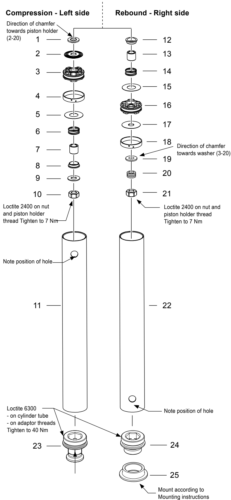
Figure 3 - Damping unit
