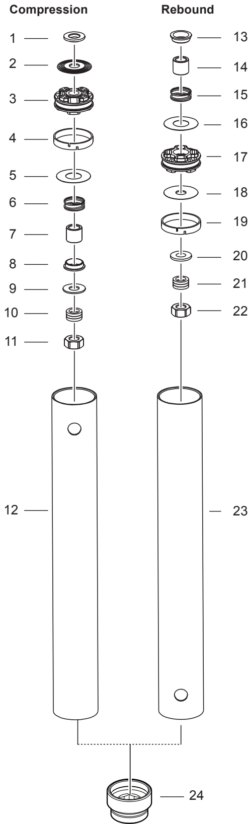
Figure 3 - Damping unit
