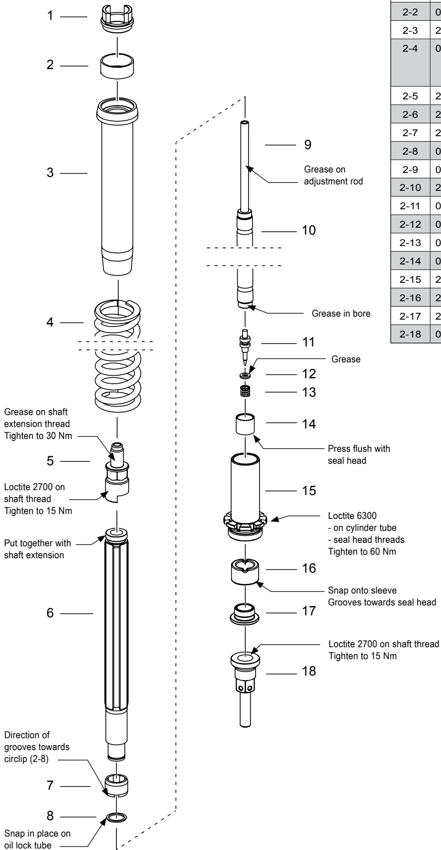
Figure 2 - Shaft assembly
