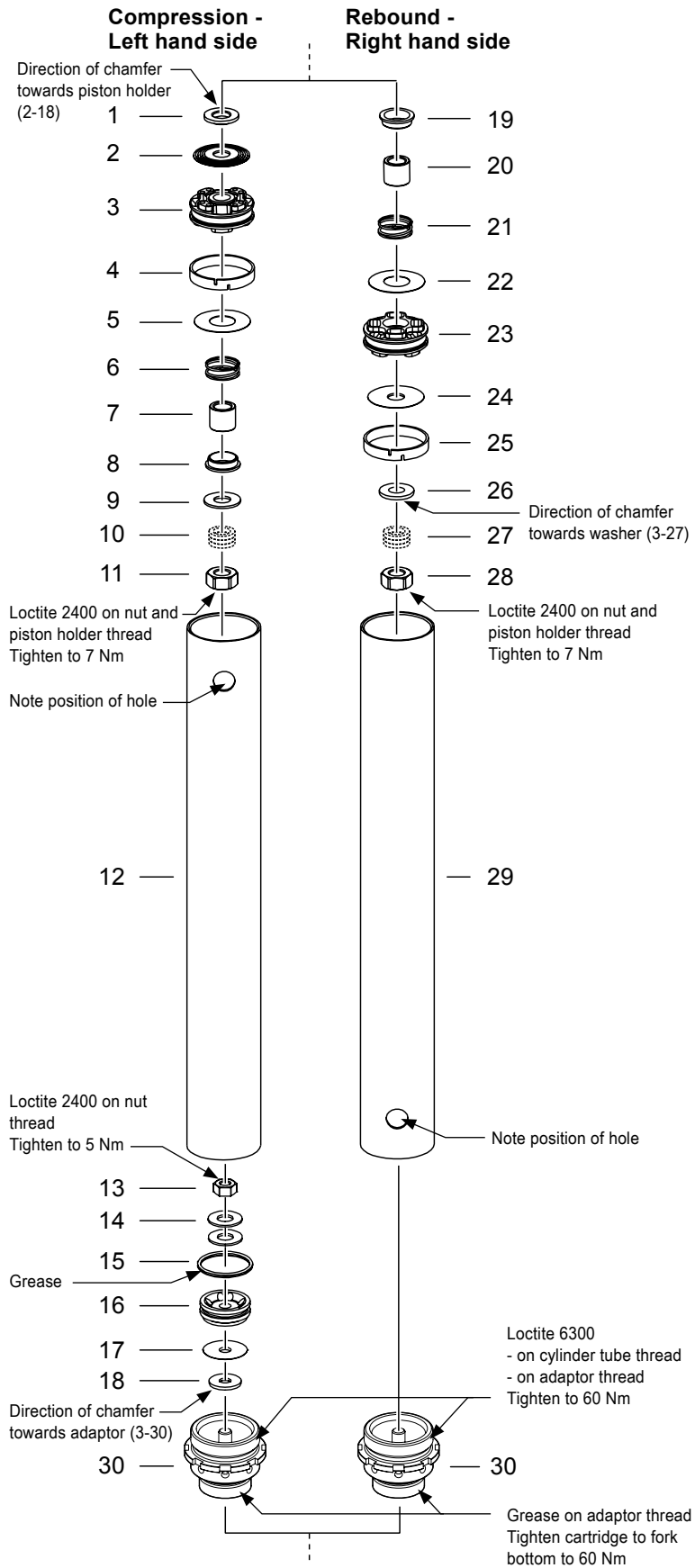
Figure 3 - Damping unit
