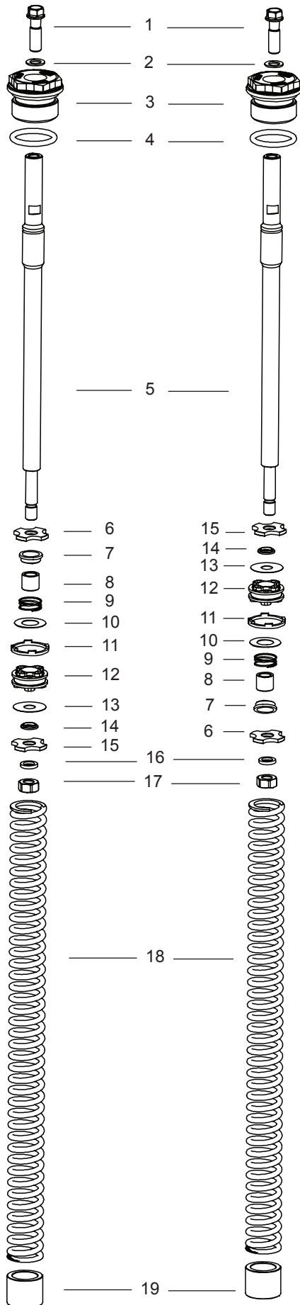
Figure 1 - Damping assy
