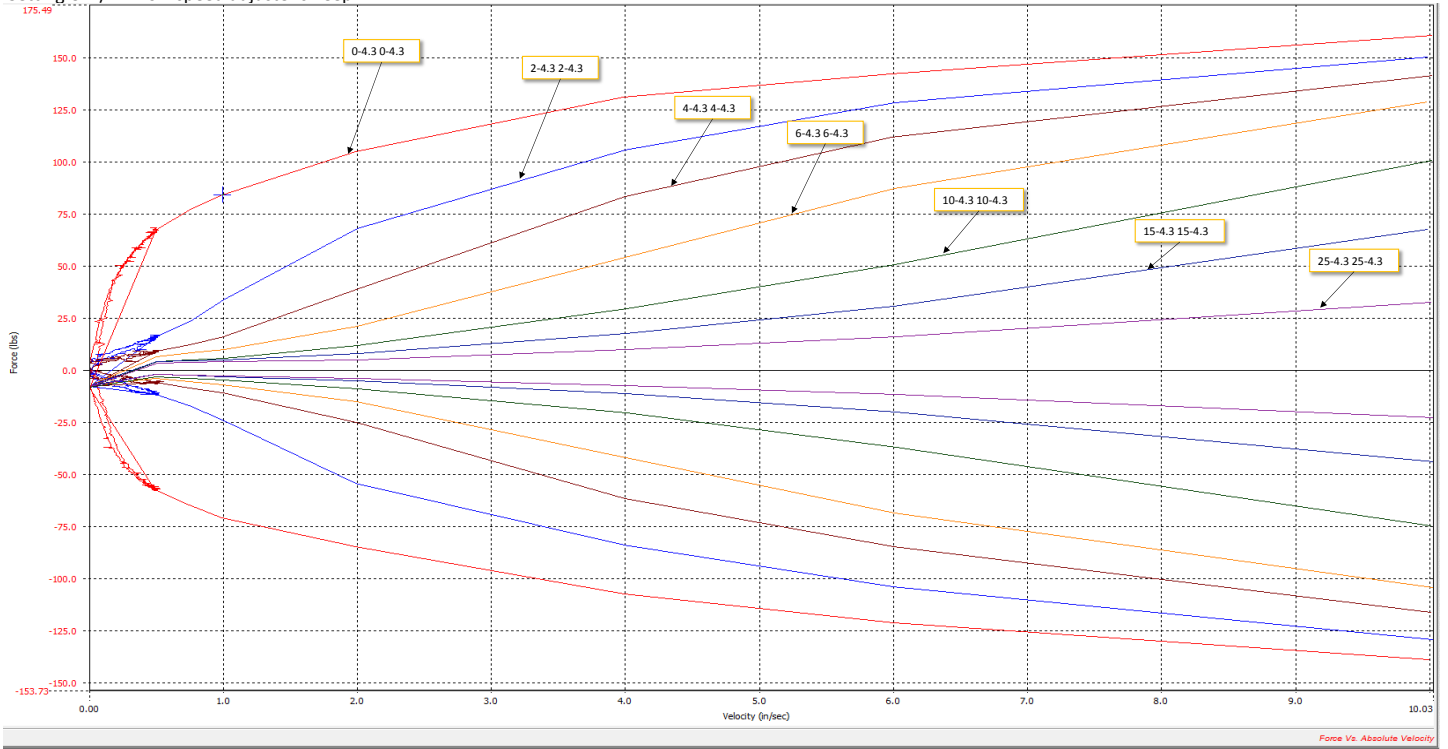
Setting C12/R12 low speed adjuster sweep
